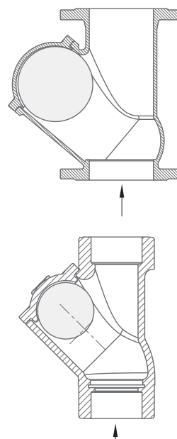
FIGURE 2. VERTICAL INSTALLATION
