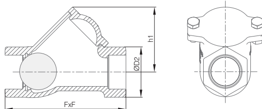
FIGURE 4. THREADED CONNECTION
