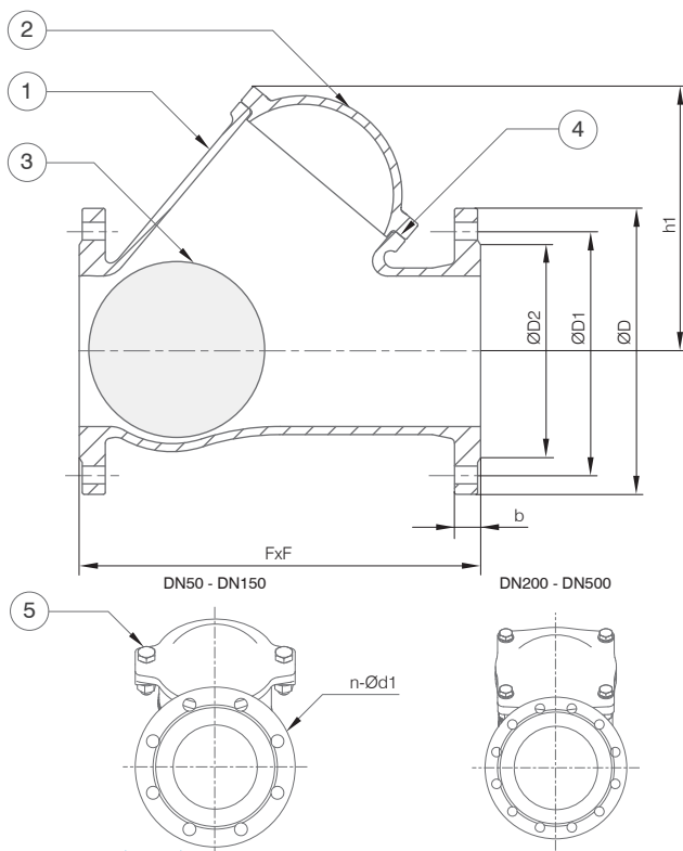
FIGURE 3. FLANGED CONNECTION
